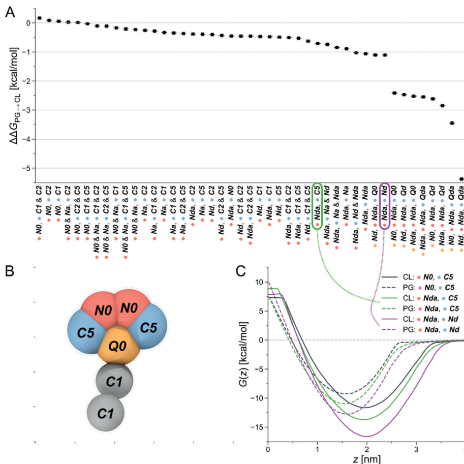
Fig. 2 Computational selection of SM_{1-22} . (A) Differences in partitioning free energies \Delta\Delta G_{PG \rightarrow CL} from alchemical transformations of one or more beads in the CG-representation of NAO. (B) Original CG representation of NAO color-coded to visualize the locations of bead changes in the free energy calculations. (C) Exemplary PMFs of CG structures with different bead types in the CL membrane (solid lines) and the PG membrane (dashed lines). Connections show which PMF curve corresponds to which partitioning free energy difference \Delta\Delta G_{PG \rightarrow CL} .
