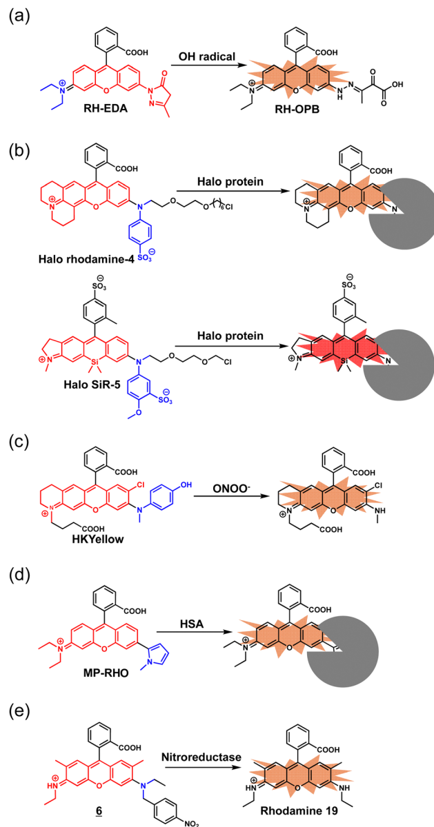
Fig. 10 TICT-based fluorogenic probes having the rhodamine scaffold. (a) Probe with modification of the N atom on the xantheno ring. (b) Ph-rhodamine-based probes for the detection of HaloTag protein. (c) Probe utilizing a phenol moiety. (d) Probe utilizing a pyrrole moiety. (e) Probe employing the sr-TICT mechanism.
