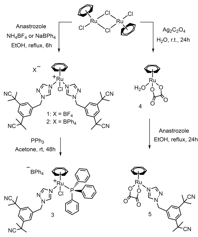
Scheme 1. Synthetic Route to Complexes 1–5
