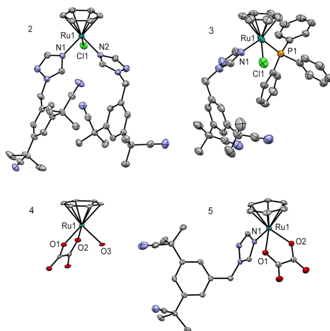
Figure 1. ORTEP diagrams (showing thermal ellipsoids at the 50% probability level) of complexes 2–5 . Note that in the case of 3 , only one site is shown for the disordered benzene, Cl and CN. 2 : Ru1–N1, 2.1024(12) Å; Ru1–N2, 2.1104(12) Å. 3 : Ru1–N1, 2.114(4); Ru1'–N1', 2.091(5). 5 : Ru1–N1, 2.1130(15) Å.
