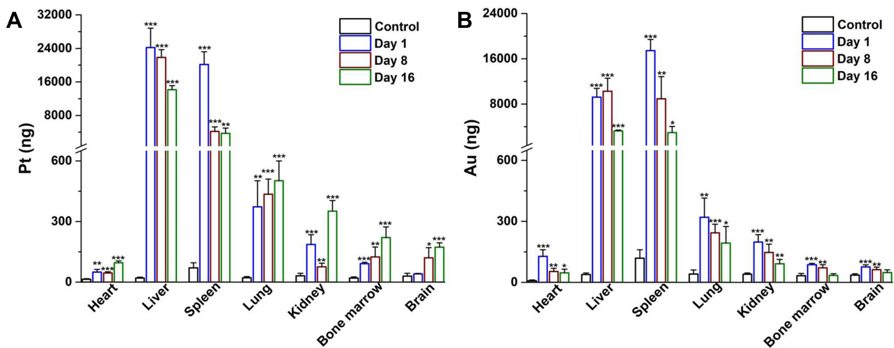
Figure 3 The distribution of (A) Pt and (B) Au in different tissue after one injection (ng). Each data represents the mean ± SD (n = 4). *Represents the significant difference compared with the control. *: 0.01 < p < 0.05, **: 0.001 < p < 0.01, ***: p < 0.001.
