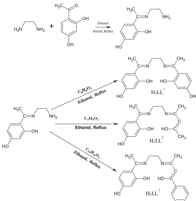
Scheme 1. Synthesis of \text{H}_2\text{LL}^1 – \text{H}_2\text{LL}^3 .
