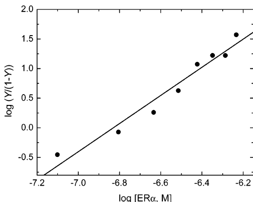
Figure 5. Hill plot for the binding of [\text{Ru}(\text{Ph}_2\text{-phen})_2(\text{mbpy-C6-est})](\text{PF}_6)_2 to ER \alpha .
