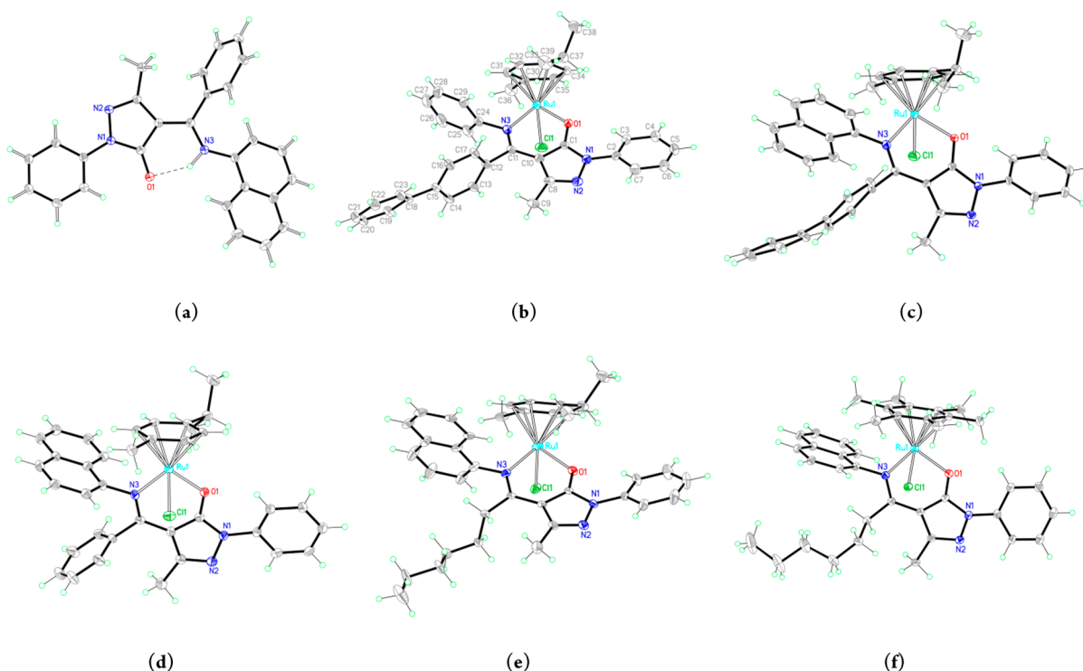
Figure 1. Molecular structures of HL ph,naph (a); 1 , [Ru(cym)(L biph,ph )Cl] (b); 4 , [Ru(cym)(L biph,naph )Cl] (c); 5 , [Ru(cym)(L ph,naph )Cl] (d); 8 , [Ru(cym)(L hex,naph )Cl] (e); and 9 , [Ru(hmb)(L hex,naph )Cl] (f). Selected bond lengths (Å) and angles (deg): HL ph,naph , C1–O1 1.255(2), N1–N2 1.406(2), N3...O1 2.698(2), N3–H3...O1 144(2); 1 , Ru1–O1 2.068(4), Ru1–N3 2.130(5), Ru1–Cl1 2.412(2), O1–Ru1–N3 87.45(18), O1–Ru1–Cl1 85.05(15), N3–Ru1–Cl1 84.39(15); 4 , Ru1–O1 2.073(2), Ru1–N3 2.148(2), Ru1–Cl1 2.420(1), O1–Ru1–N3 87.81(9), O1–Ru1–Cl1 83.67(6), N3–Ru1–Cl1 87.28(8); 5 , Ru1–O1 2.083(3), Ru1–N3 2.118(3), Ru1–Cl1 2.447(1), O1–Ru1–N3 88.74(13), O1–Ru1–Cl1 84.66(9), N3–Ru1–Cl1 83.89(10); 8 , Ru1–O1 2.070(3), Ru1–N3 2.128(4), Ru1–Cl1 2.426(1), O1–Ru1–N3 88.91(13), O1–Ru1–Cl1 84.84(10), N3–Ru1–Cl1 84.43(11); 9 , Ru1–O1 2.084(5), Ru1–N3 2.164(6), Ru1–Cl1 2.444(2), O1–Ru1–N3 89.37(19), O1–Ru1–Cl1 84.61(15), N3–Ru1–Cl1 81.67(16).
